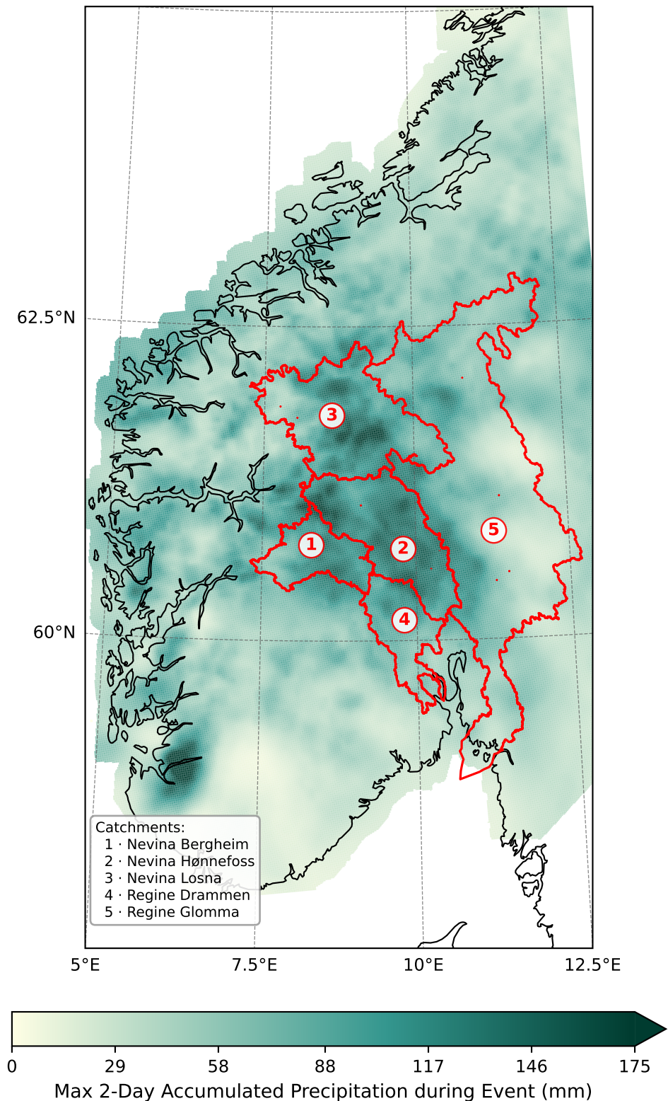
Storm Hans - Max 2-Day Precip. Envelope (7-9 Aug 2023): SeNorge/1kmx1km
