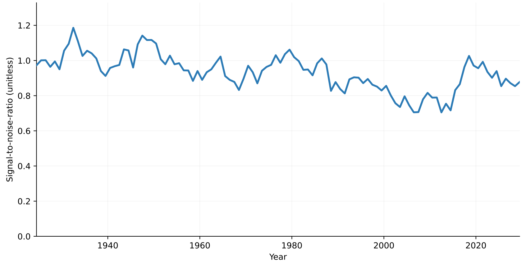
Signal-to-noise-ratio Compound (Precipitation and Snowmelt) Hazard for Regine Drammen + Glomma from 1920-2034
