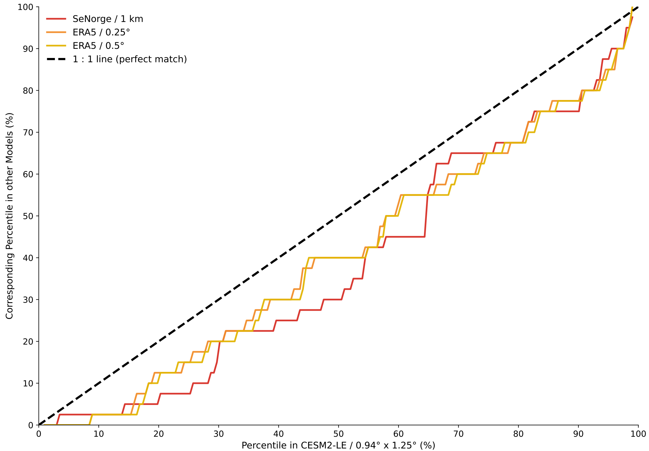
Percentile Mapping of Annual Maximal 1-day Accumulated Precipitation — Regime Glomma
