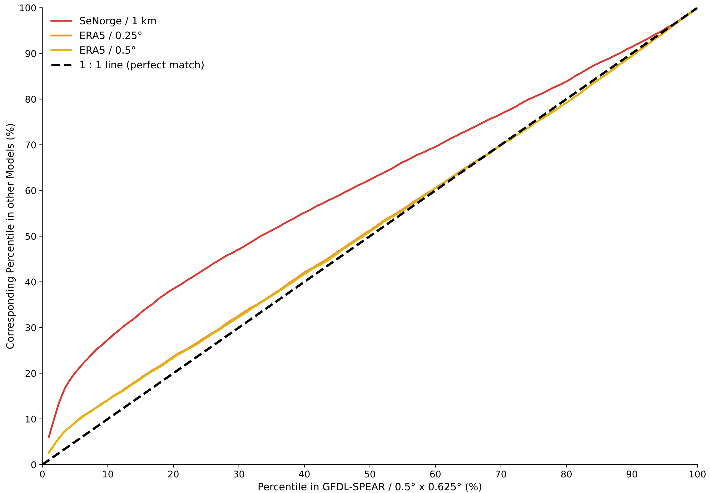
Percentile Mapping of Daily 2-day Accumulated Precipitation — Nevina Losna
