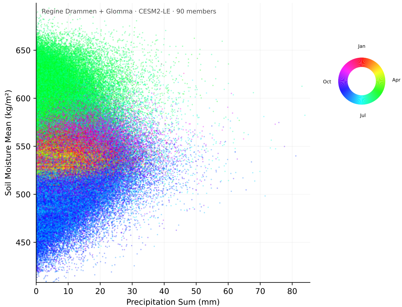
Joint Distribution of 2-Day Precipitation Sum and 2-Day Soil-Moisture Mean, 1995-2024
