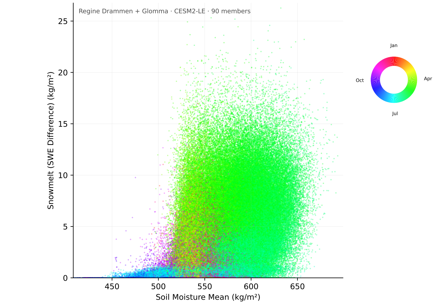
Joint Distribution of 2-Day Soil-Moisture Mean and 2-Day Snowmelt (SWE Difference), 1995-2024
