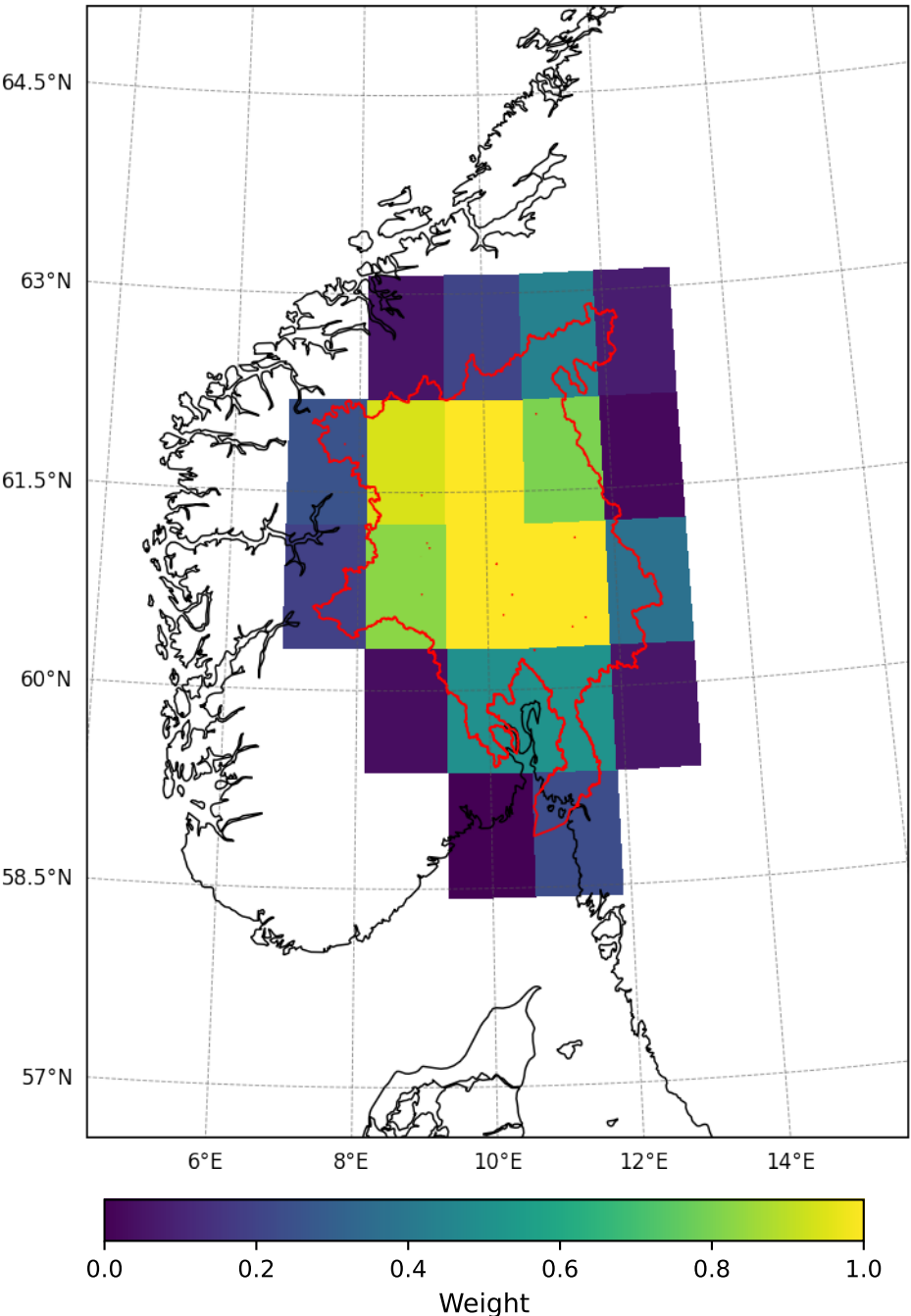
Catchment Weights: CESM2-LE/0.94x1.25 — Regime Drammen + Glomma
