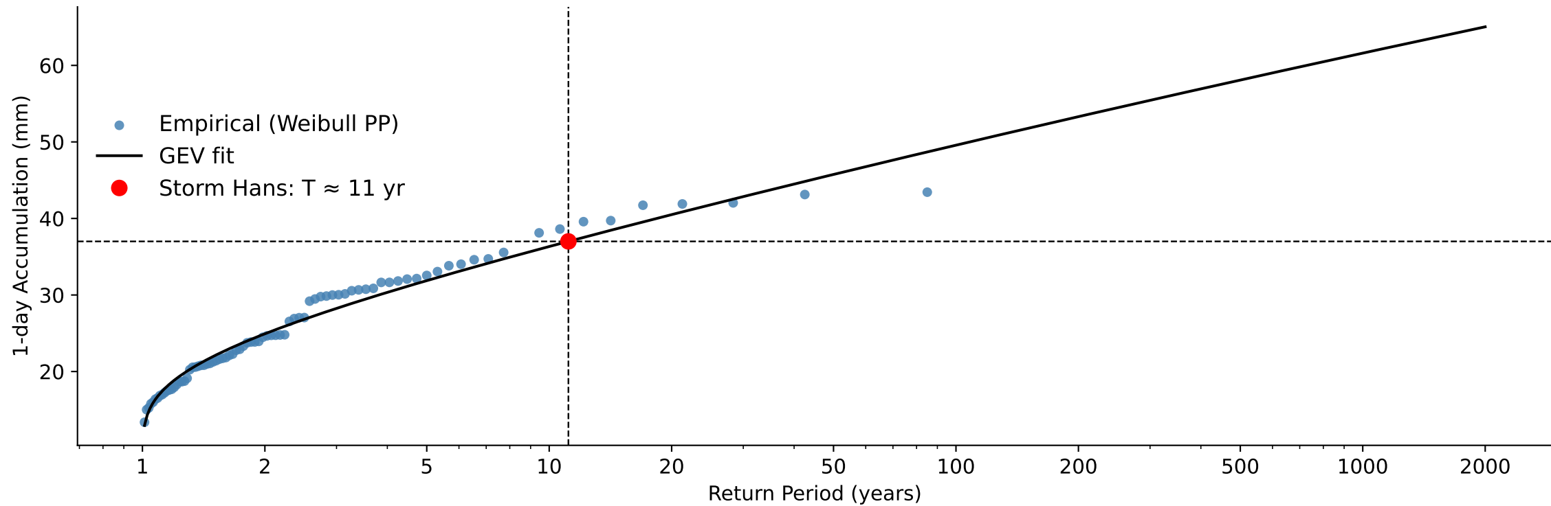
B) Weighted Catchment 1-day Accumulated Precipitation, Return Period Storm Hans: 11 year
