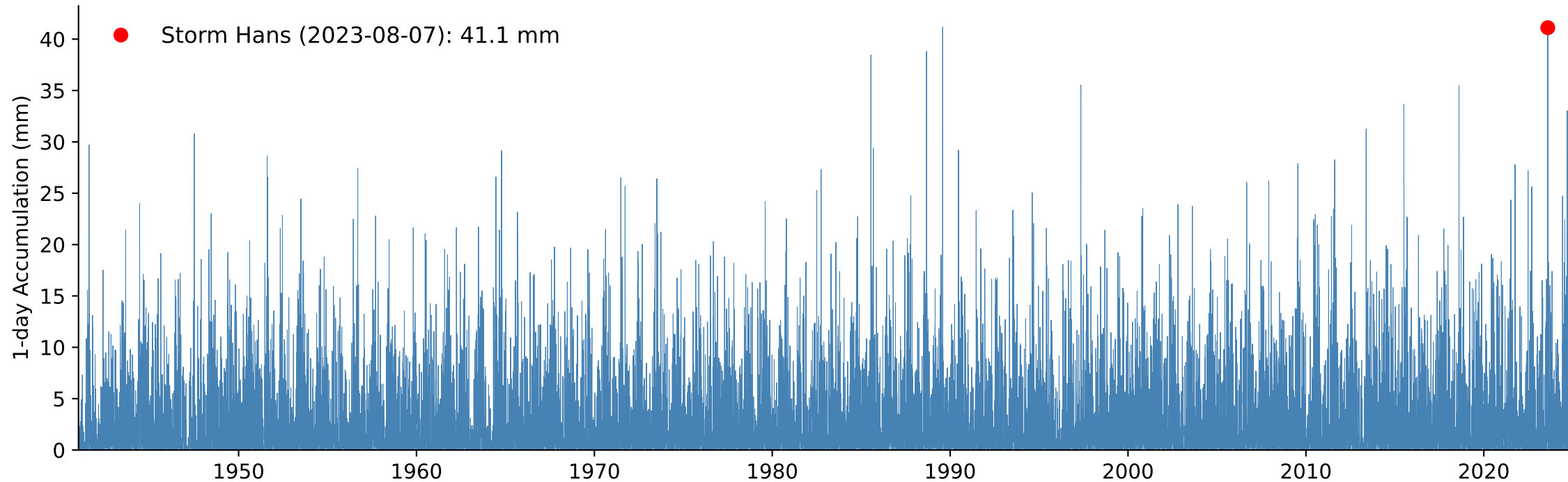
B) Weighted Catchment 1-day Accumulated Precipitation, Return Period Storm Hans: 43 year
