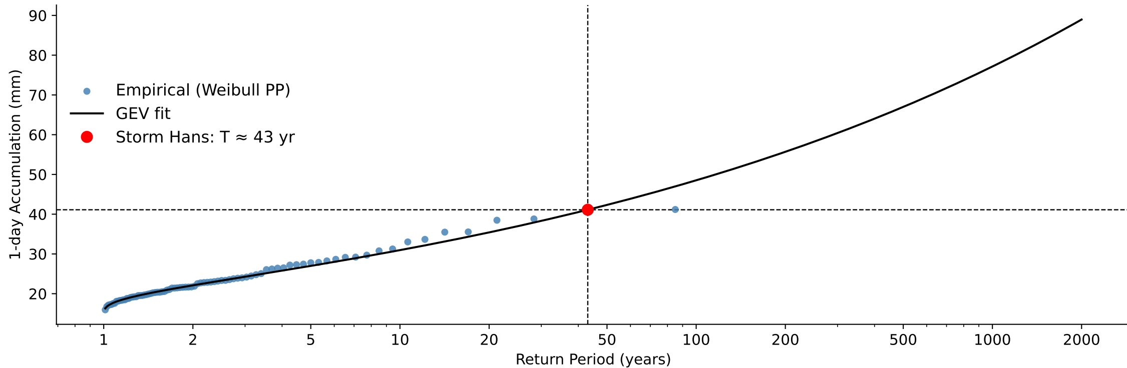
B) Weighted Catchment 1-day Accumulated Precipitation, Return Period Storm Hans: 43 year
