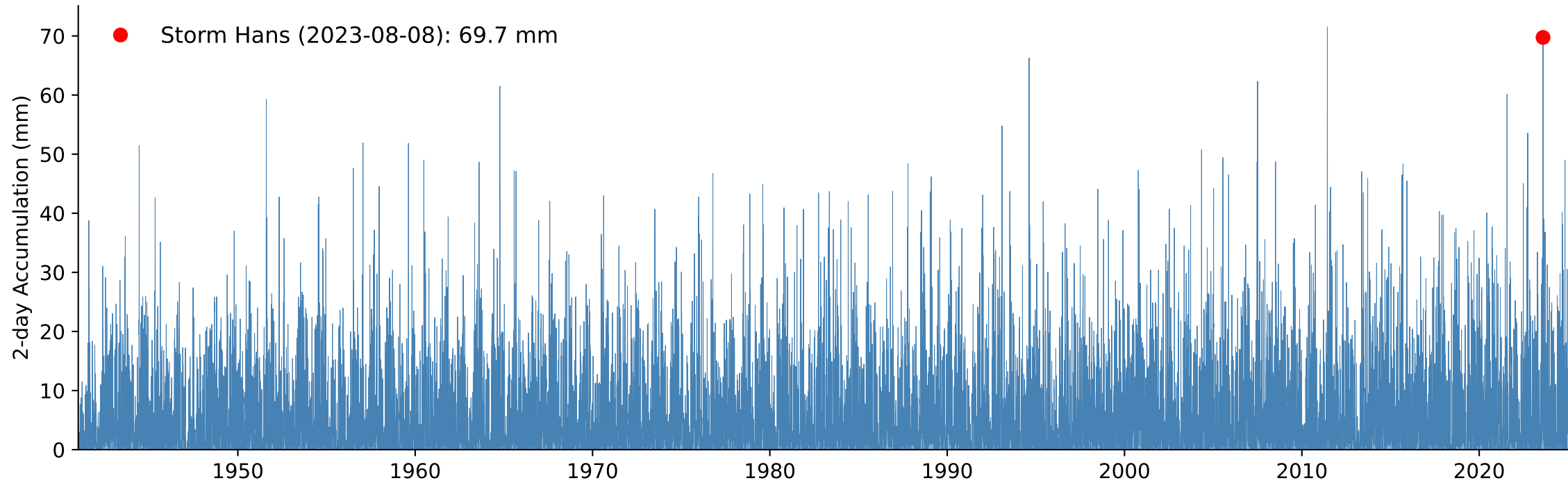
B) Weighted Catchment 2-day Accumulated Precipitation, Return Period Storm Hans: 101 year
