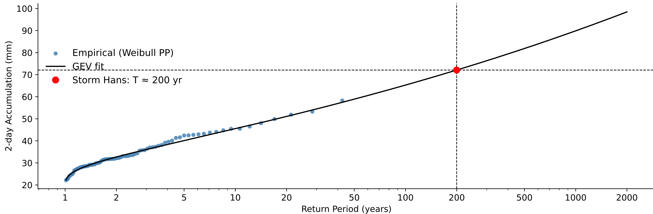
B) Weighted Catchment 2-day Accumulated Precipitation, Return Period Storm Hans: 200 year
