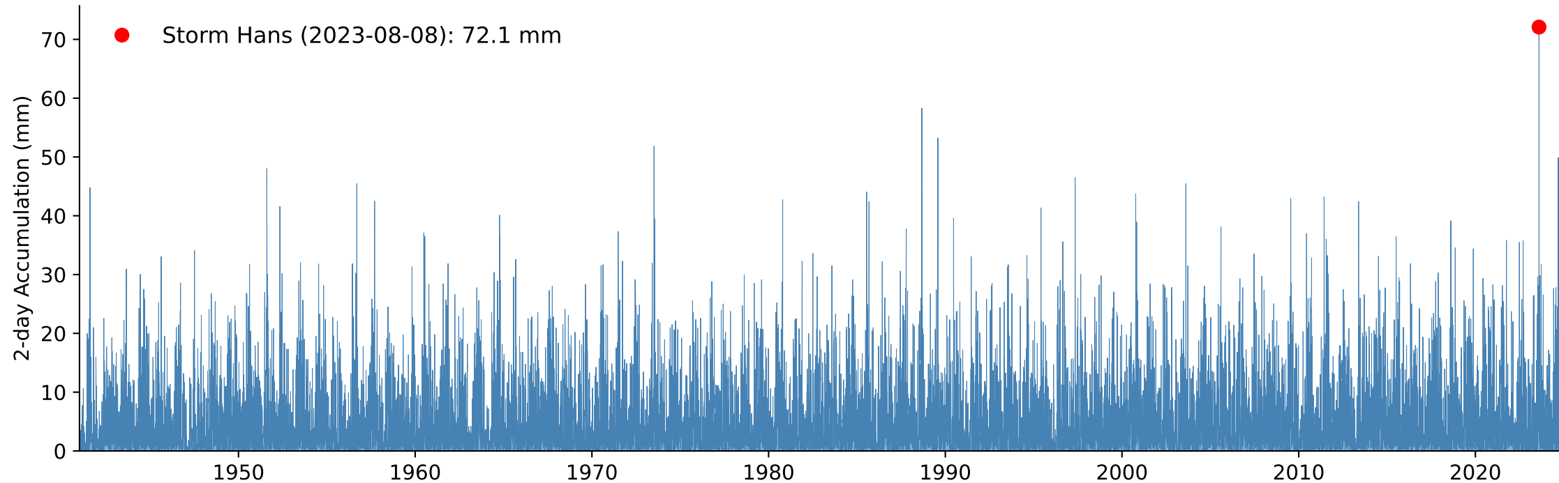
B) Weighted Catchment 2-day Accumulated Precipitation, Return Period Storm Hans: 200 year
