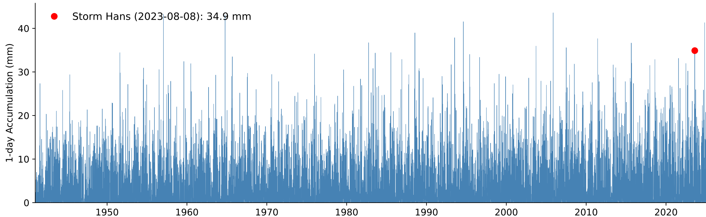
B) Weighted Catchment 1-day Accumulated Precipitation, Return Period Storm Hans: 6 year
