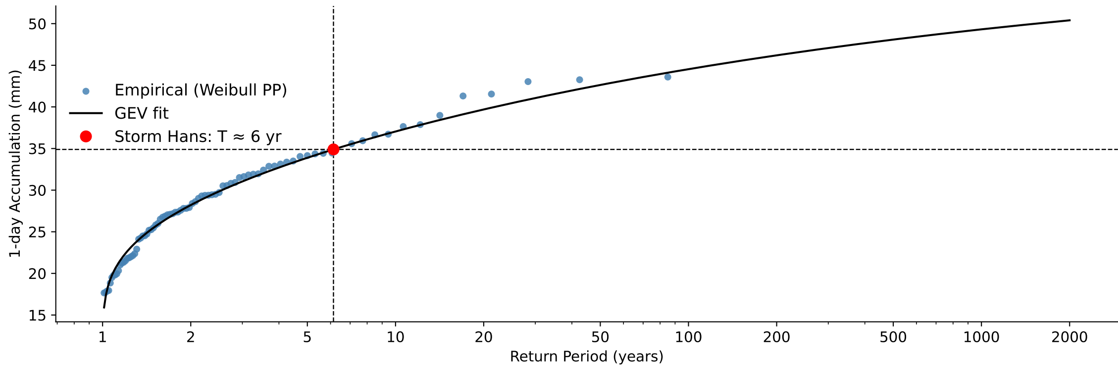
B) Weighted Catchment 1-day Accumulated Precipitation, Return Period Storm Hans: 6 year
