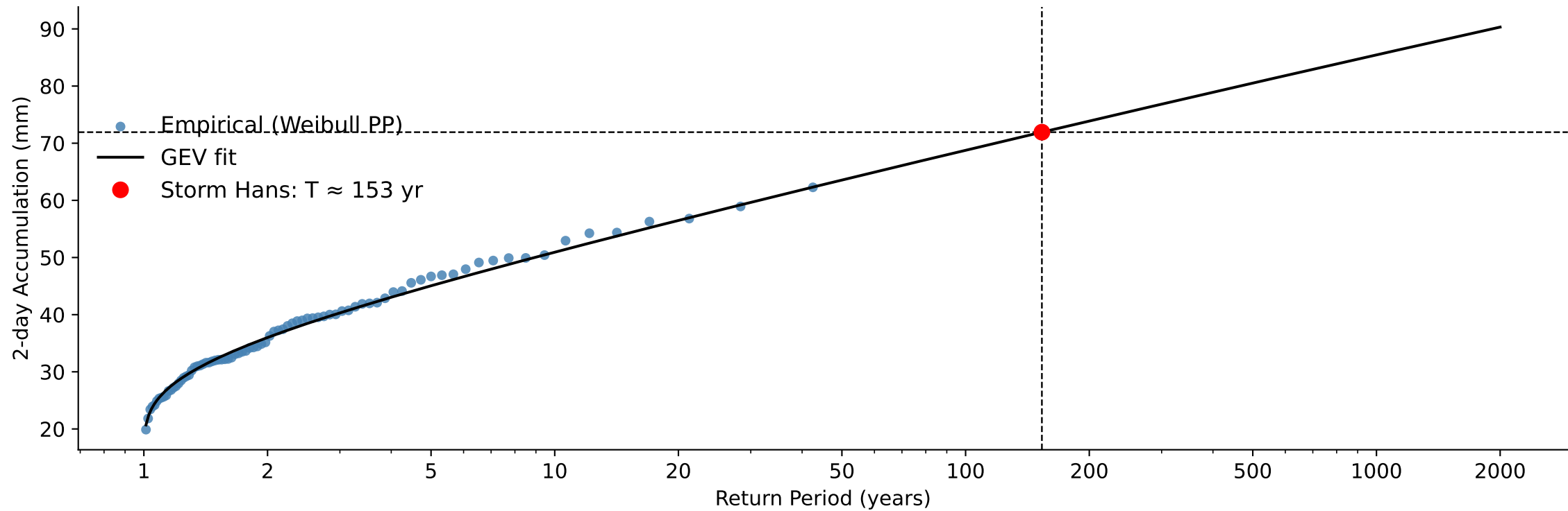
B) Weighted Catchment 2-day Accumulated Precipitation, Return Period Storm Hans: 153 year
