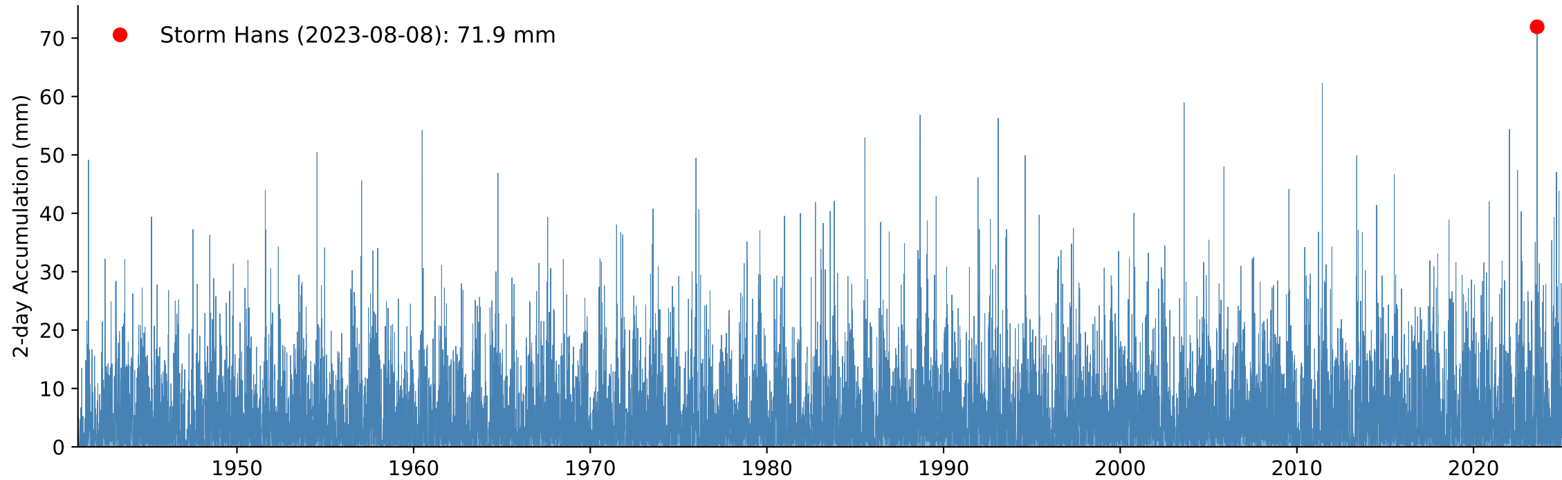
B) Weighted Catchment 2-day Accumulated Precipitation, Return Period Storm Hans: 153 year
