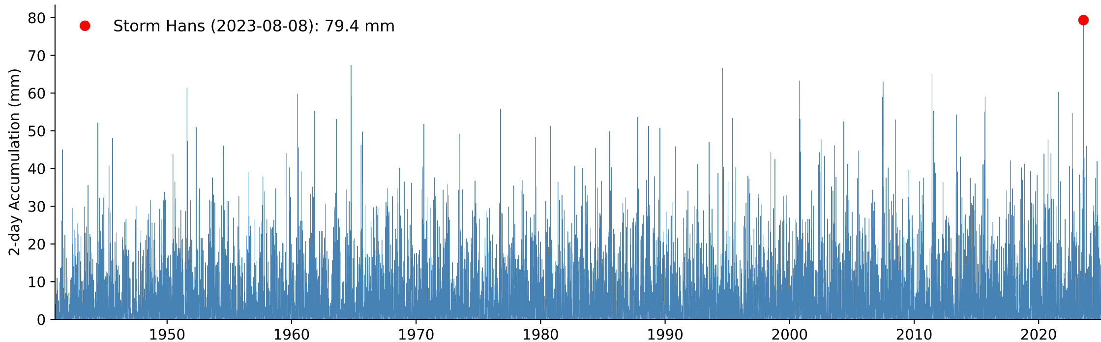
B) Weighted Catchment 2-day Accumulated Precipitation, Return Period Storm Hans: 138 year
