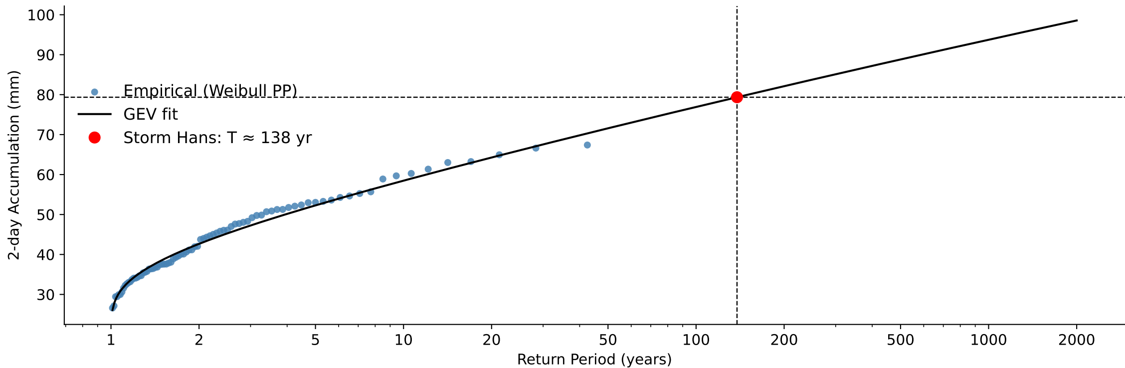
B) Weighted Catchment 2-day Accumulated Precipitation, Return Period Storm Hans: 138 year
