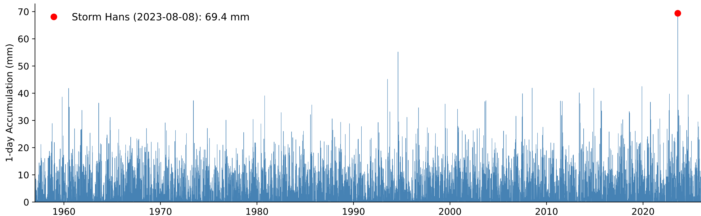
B) Weighted Catchment 1-day Accumulated Precipitation, Return Period Storm Hans: 225 year
