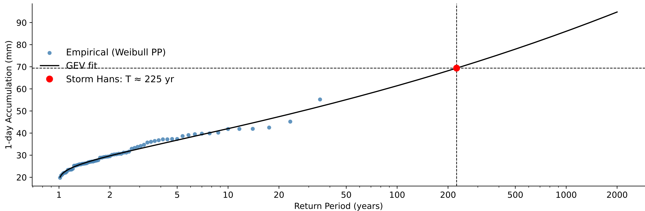
B) Weighted Catchment 1-day Accumulated Precipitation, Return Period Storm Hans: 225 year
