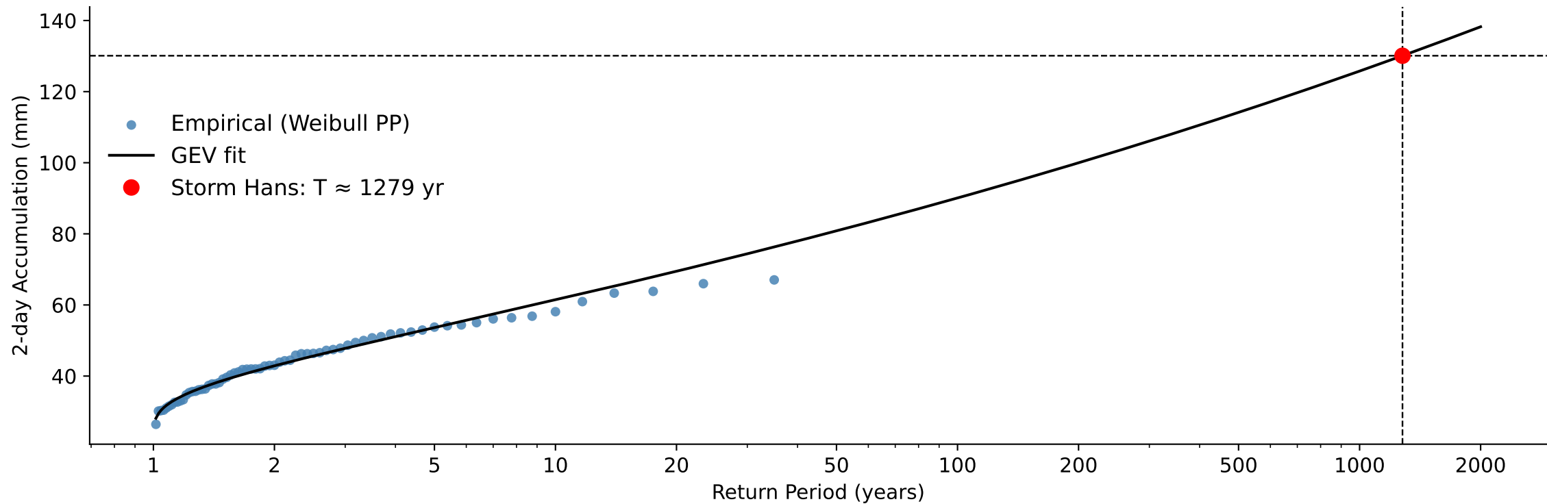
B) Weighted Catchment 2-day Accumulated Precipitation, Return Period Storm Hans: 1279 year
