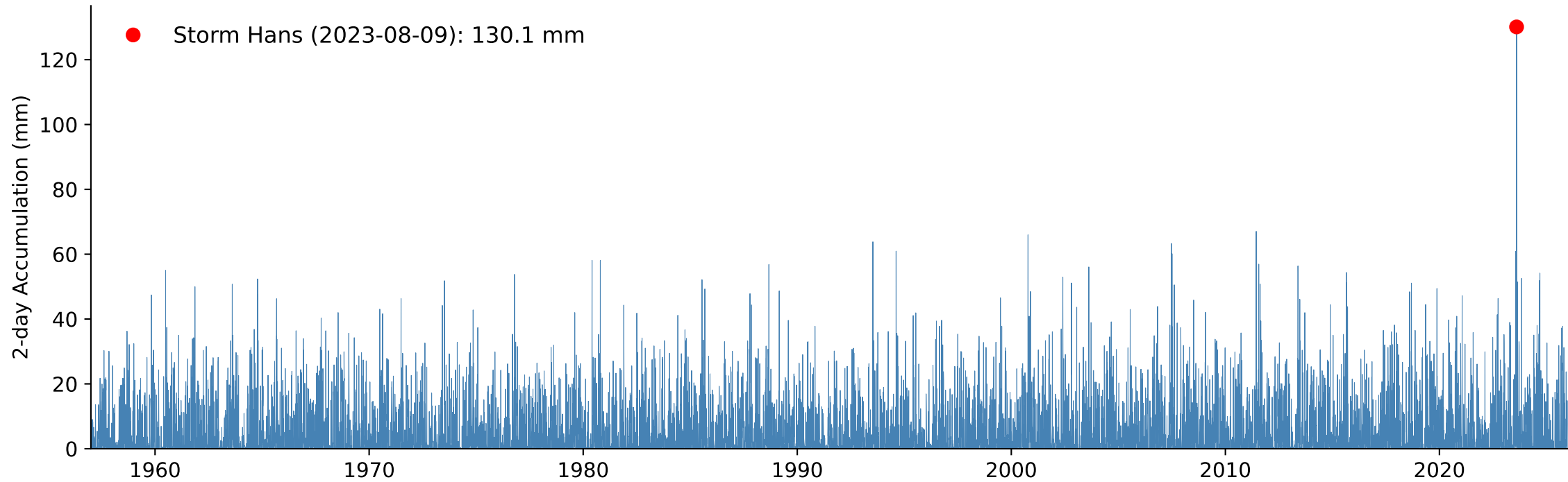
B) Weighted Catchment 2-day Accumulated Precipitation, Return Period Storm Hans: 1279 year
