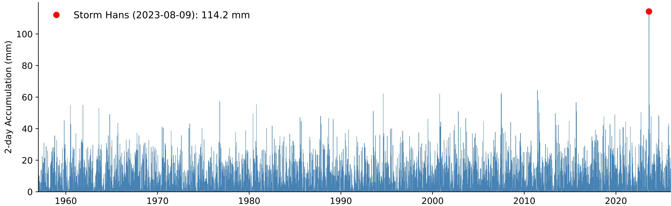
B) Weighted Catchment 2-day Accumulated Precipitation, Return Period Storm Hans: 797 year
