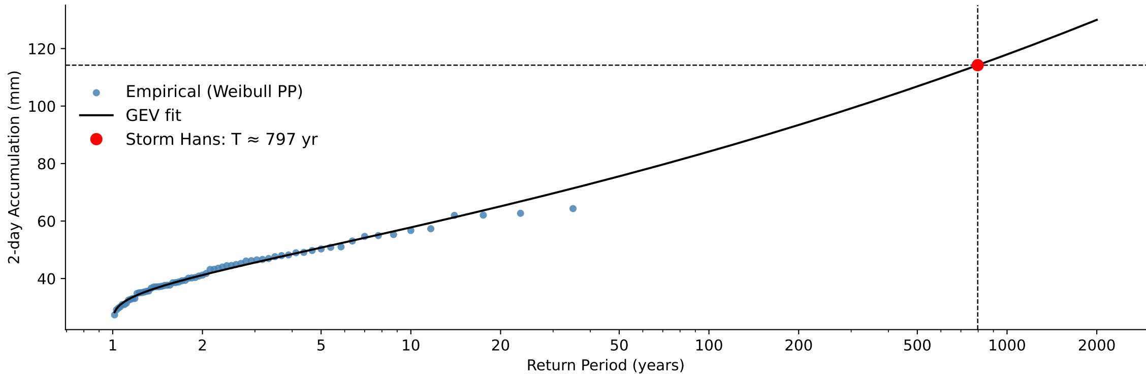
B) Weighted Catchment 2-day Accumulated Precipitation, Return Period Storm Hans: 797 year
