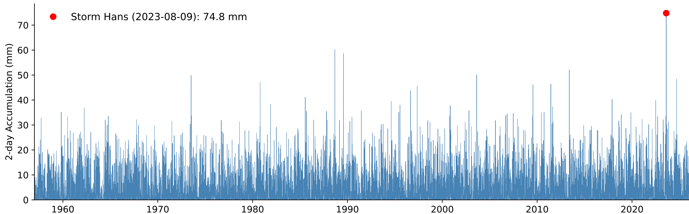
B) Weighted Catchment 2-day Accumulated Precipitation, Return Period Storm Hans: 149 year
