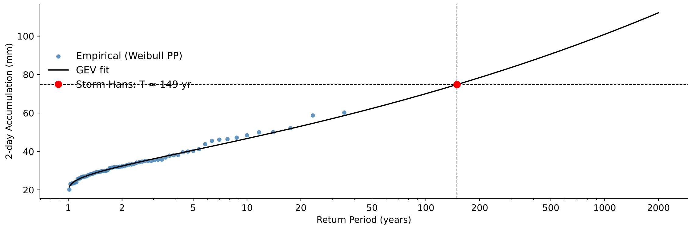
B) Weighted Catchment 2-day Accumulated Precipitation, Return Period Storm Hans: 149 year
