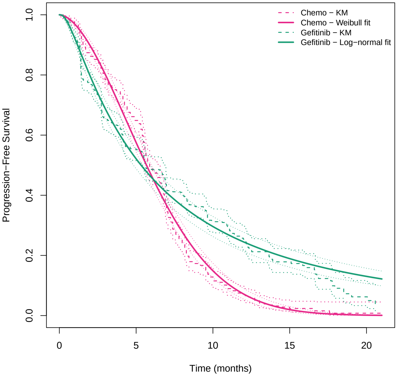
Arm-specific Parametric Fits vs KM
