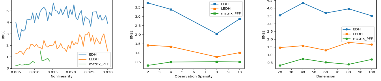
Figure 18: A comparison among EDH, LEDH, and matrix PFF (left: nonlinearity; middle: observation sparsity; right: dimension).
