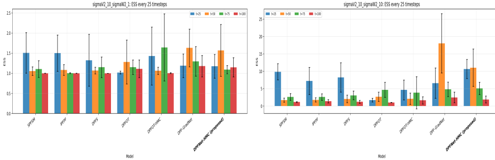
Figure 2: ESS across time steps for two scenarios for each model (left: \sigma_W^2 = 1 ; right: \sigma_W^2 = 10 )
