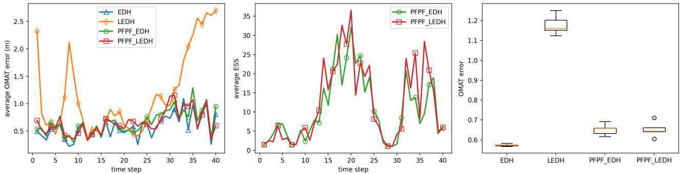
Figure 16: Main results replicated in the multi-target acoustic tracking example [Li and Coates, 2017] (left: Average OMAT errors at each time; middle: Average effective sample size at each time; right: boxplots of average OMAT error )
