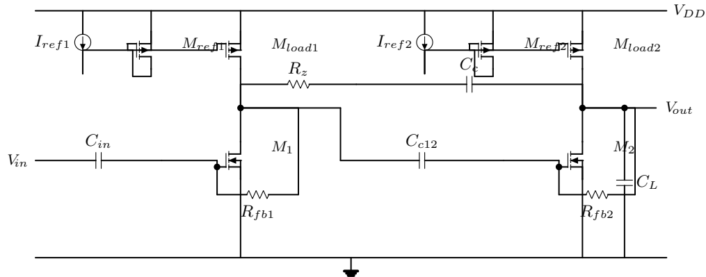
(b) cs_se_miller n = 14, d_\xi = 26
