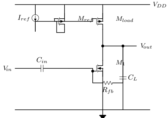
(a) cs_amp n = 6, d_\xi = 10
