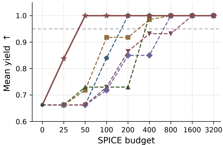
3-stage miller ( n = 22, d_{\xi} = 38 )
