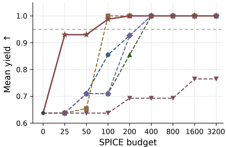
2-stage miller ( n = 14, d_{\xi} = 26 )
