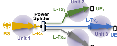
Fig. 8 – Scale to multi-units. A power splitter directs an incoming signal to multiple output units, enabling independently steered beams to serve several users simultaneously.
