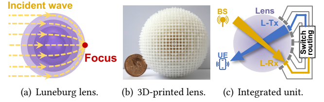
Fig. 2 – OrbWeaver architecture. The architecture of Luneburg lens and its signal focusing capability (a); the 3D-printed realization of lens (b); and integrated lens-antenna-fabricated OrbWeaver [18, 19], with a simple reflective configuration.
