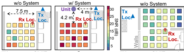
Fig. 13 – SNR gain enhancement through reflective mode.
