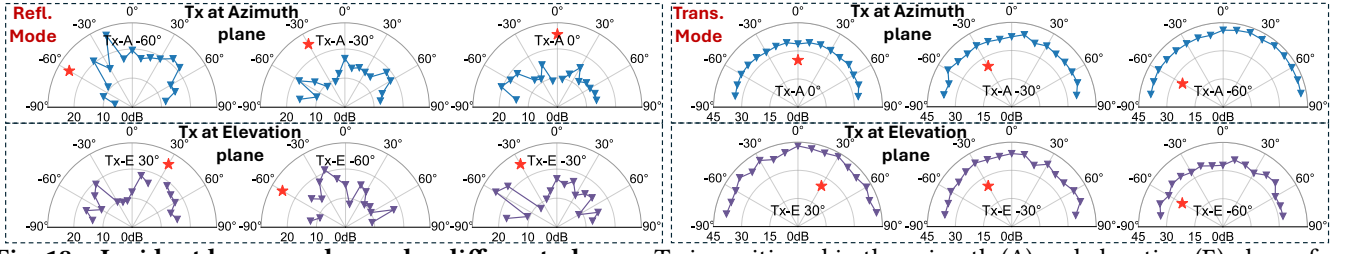
Fig. 18 – Incident beam angles under different planes: Tx is positioned in the azimuth (A) and elevation (E) planes for reflective mode (left) and transmissive mode (right). The transmitter is marked with a red star, and the receiver is measured at different angles from -80^\circ to 80^\circ with the angular resolution of 10^\circ .
