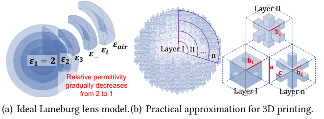
(a) Ideal Luneburg lens model. (b) Practical approximation for 3D printing.
