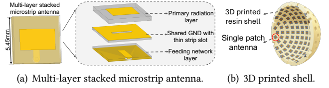
Fig. 4 – Hemisphere antenna array architecture and implementation.
