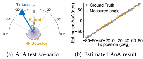
Fig. 12 – Evaluation of Tx beam AoA accuracy.
