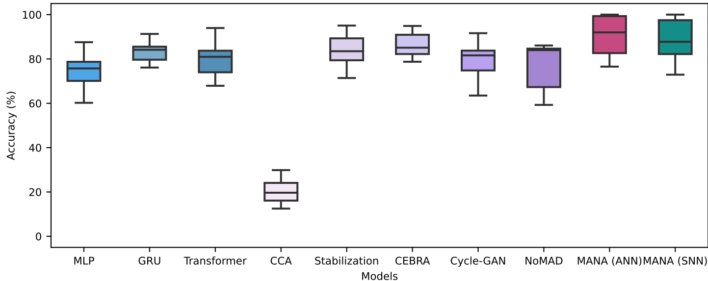
benchmark models, finetuned, phase 1
