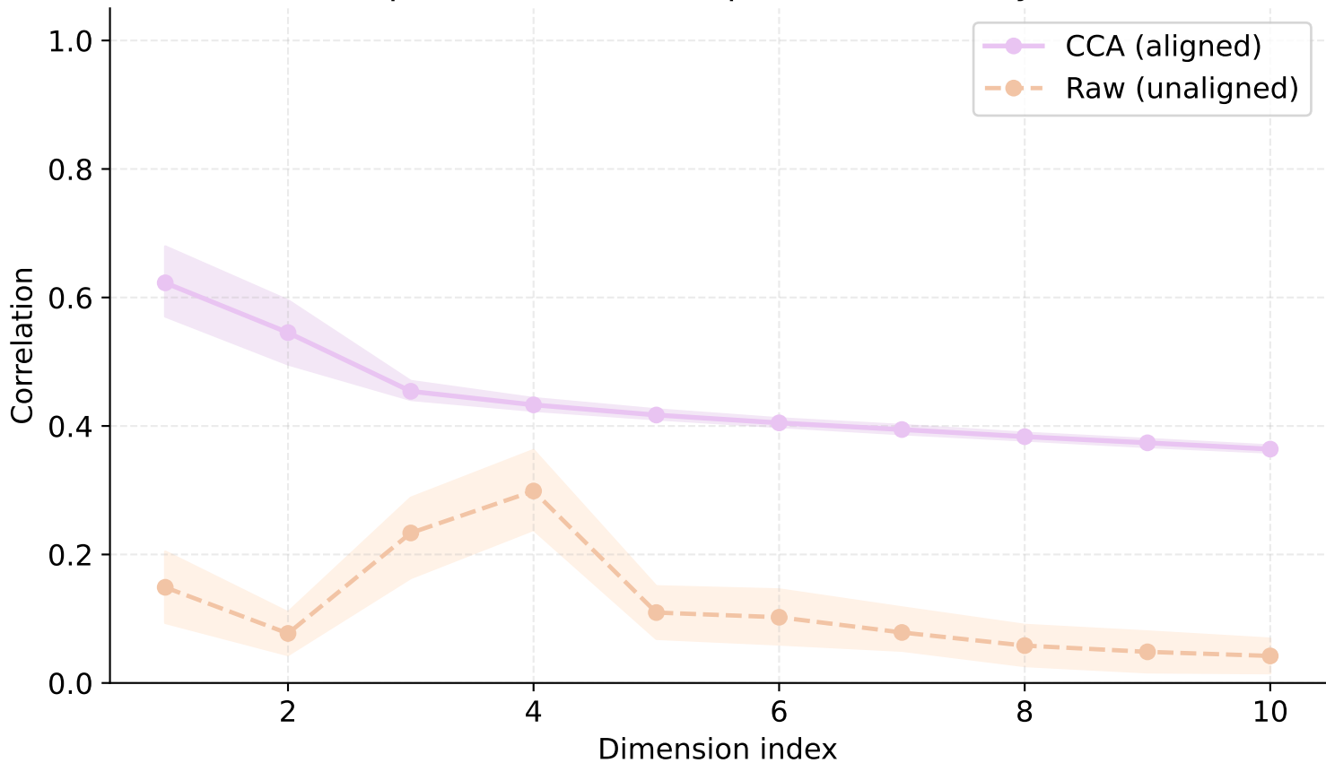
CCA Spectrum vs Raw (Top 10) — 50 \leq \text{Day} \leq 119
