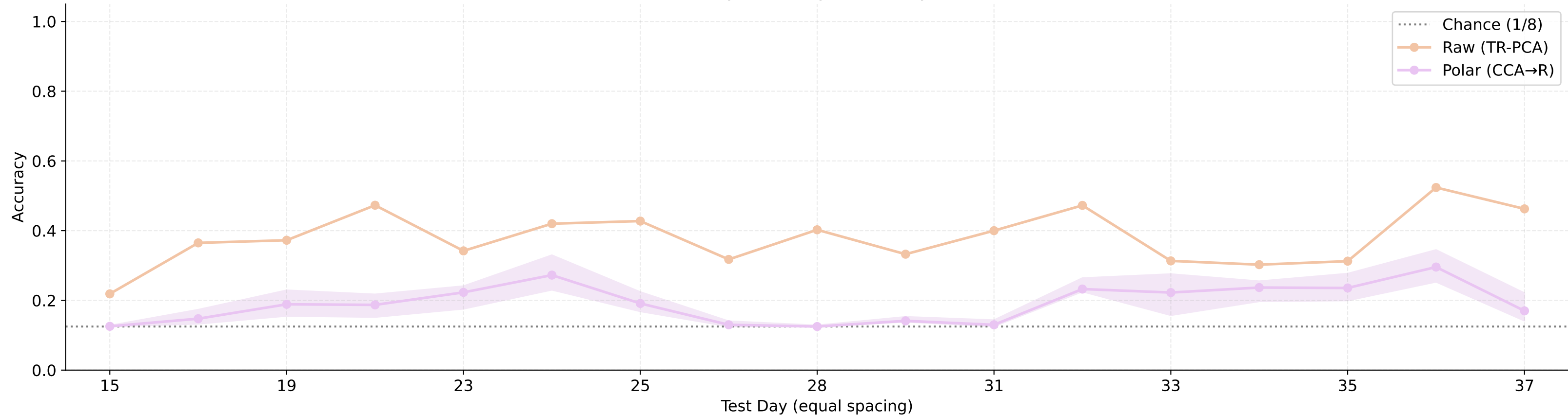
Cross-day Accuracy ( 15 \leq \text{Day} \leq 37 )
