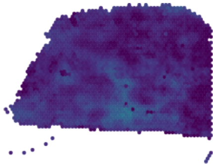
ALB | Prior ensemble r=0.282
