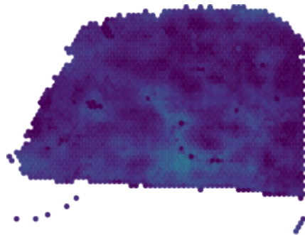
ALB | Final ensemble r=0.267
