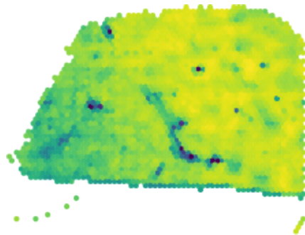
HP | Final ensemble r=0.307
