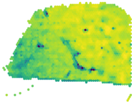
HP | Prior ensemble r=0.312
