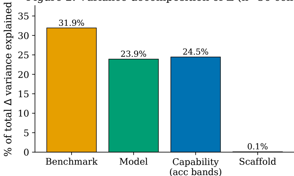
Figure 2: Variance decomposition of \Delta (n=36 cells)
