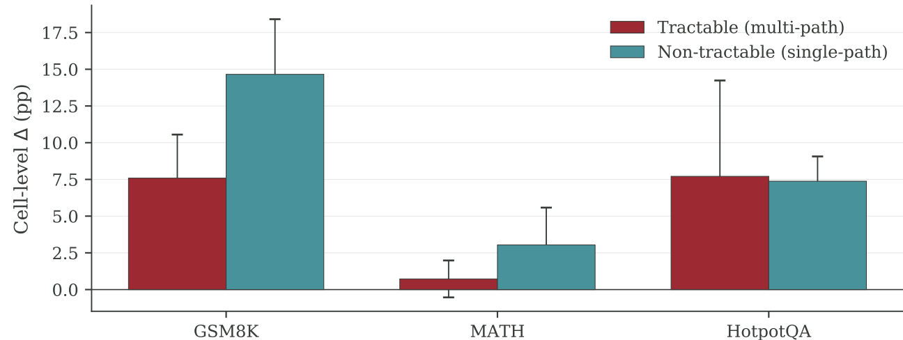
Within-benchmark tractability strata (0/3 contrasts significant)
