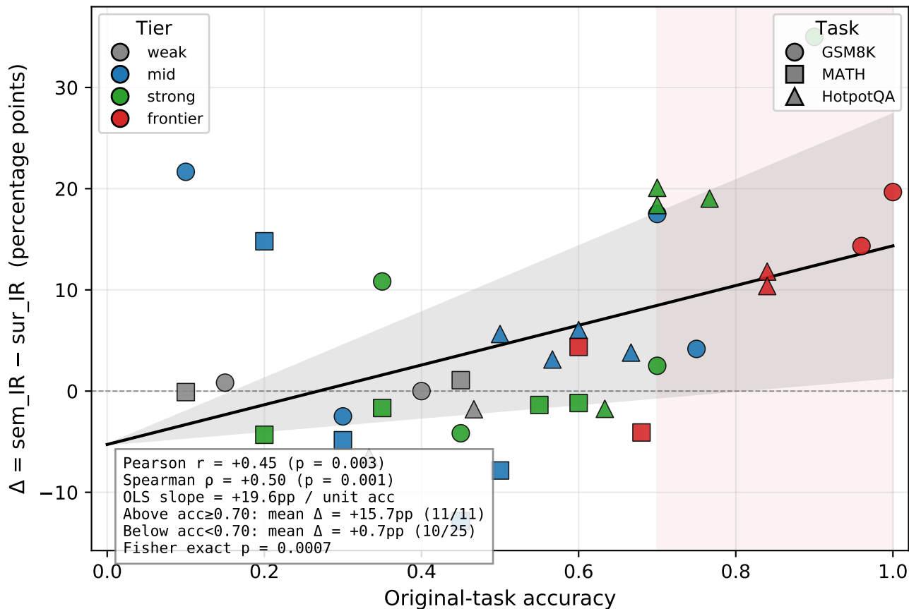
Capability-gated dichotomy: \Delta emerges with task accuracy
