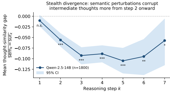
Figure 6: Per-step thought-similarity gap (sem - sur) on the qwen2.5-14B trace probe ( n=1,800 ). Step 1 is null ( p=0.12 ); the gap opens at step 2 and remains highly significant through step 6. The pattern is consistent with stealth divergence : a semantic perturbation does not change the model’s first surface action — it silently corrupts intermediate thought content from step 2 onward, and that corruption cascades 0.17 steps deeper than a presentation-level edit (M3).
