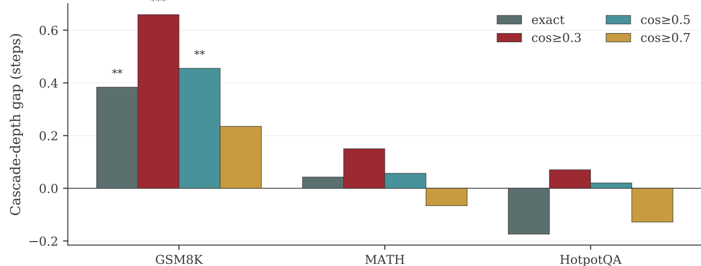
Cascade-depth gap, exact vs TF-IDF cosine; * p < .05 , ** p < .01 , *** p < .001
