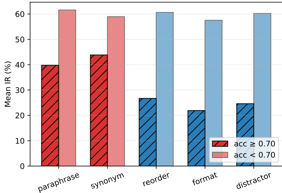
(b) Per-type IR split by capable / incapable cells ( T=0.70 )
