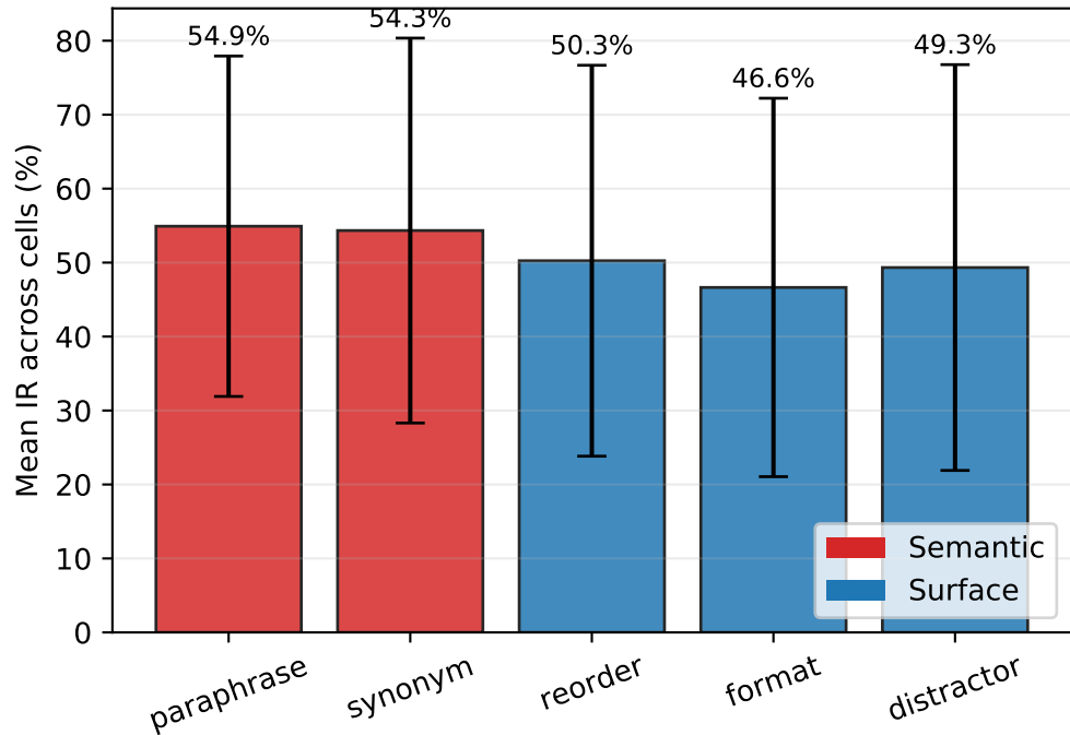
(a) Per-type IR (mean \pm SD across cells)
