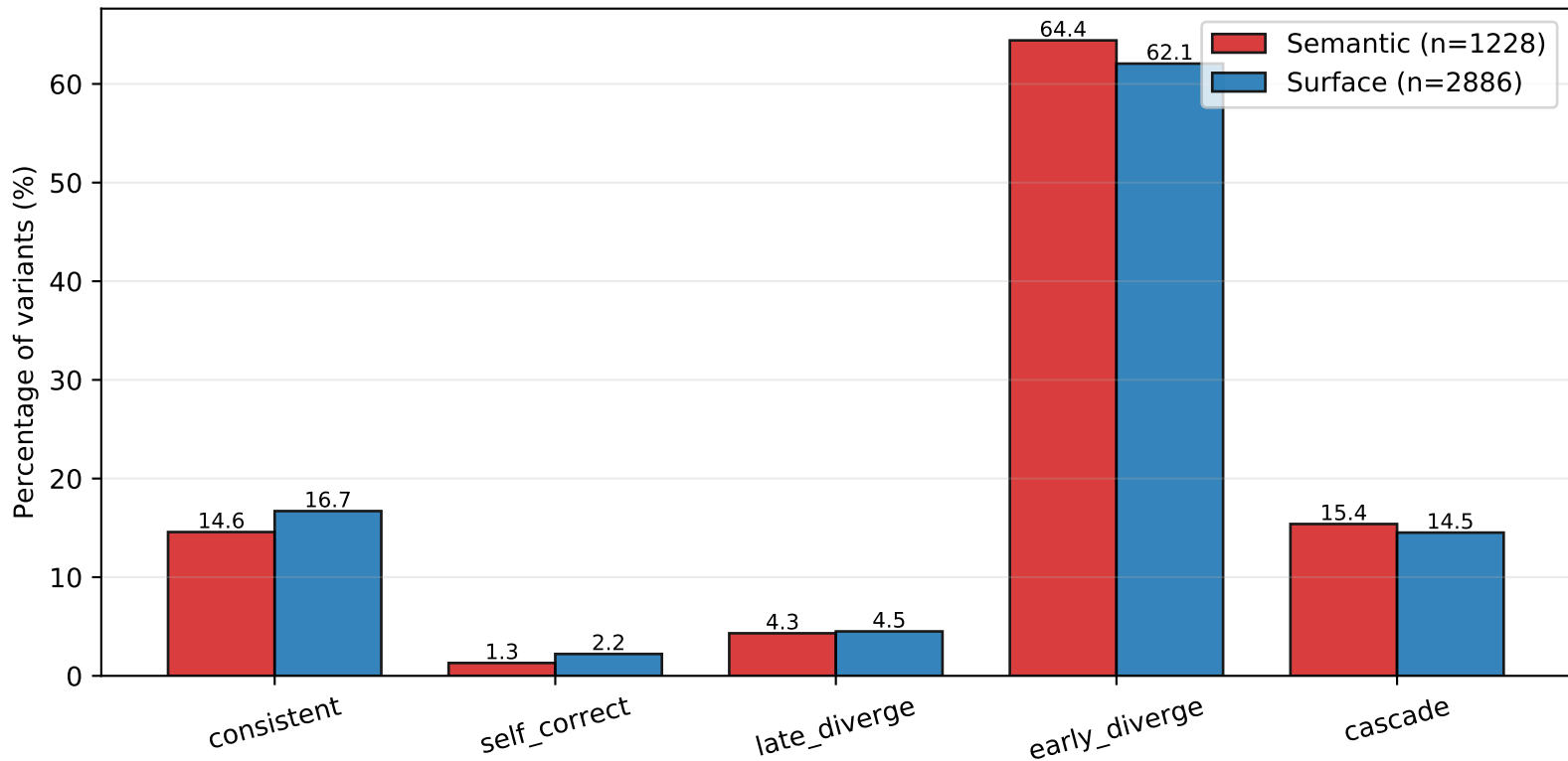
How agents fail: semantic vs surface propagation patterns ( \chi^2=7.4 , p=0.1162 )
