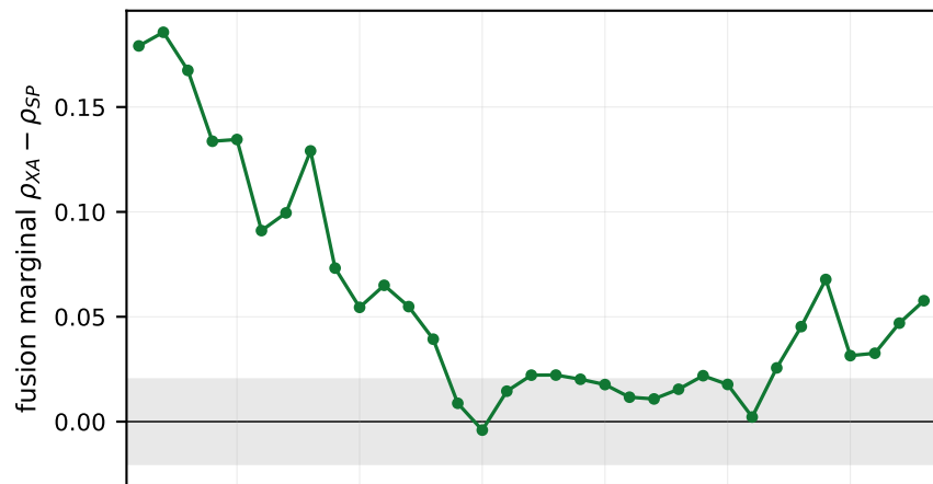
TIM (IGPS, fitness)
