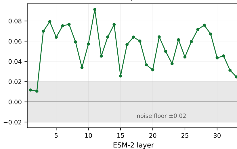
CI \lambda (expression)
