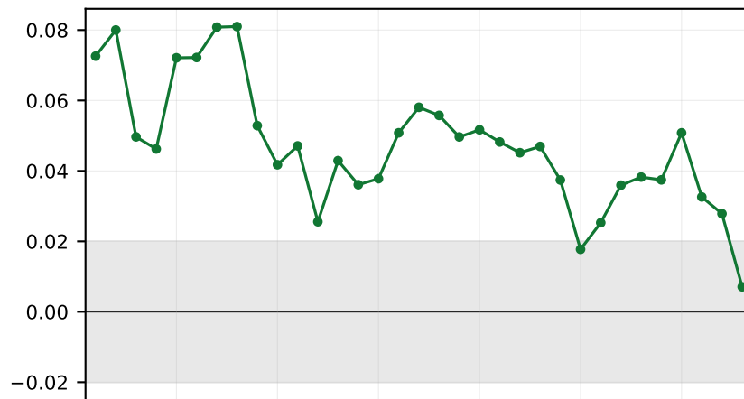
CASP3 (protease activity)
