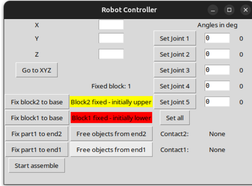
Figure 6.1: Graphical user interface for simulation control
