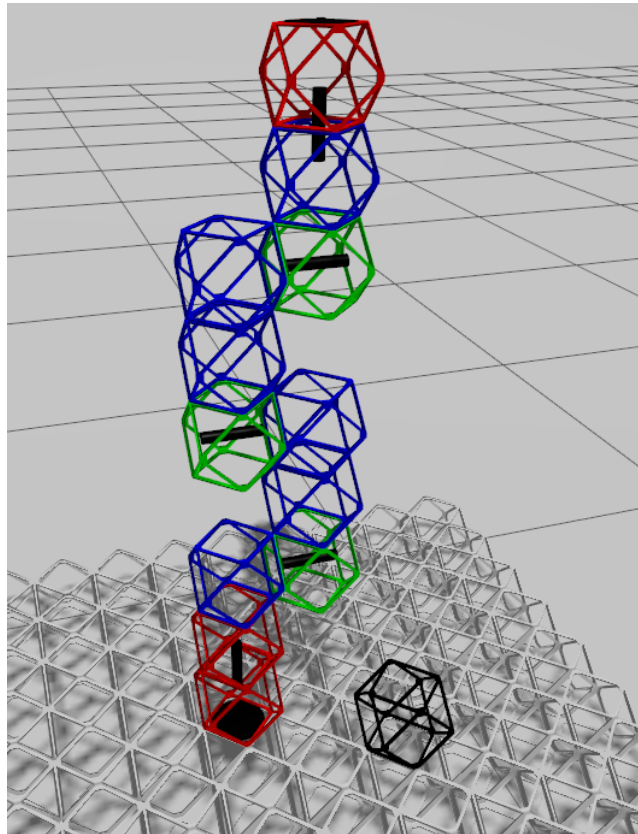
Figure 6.2: Robot structure in Gazebo simulation environment
