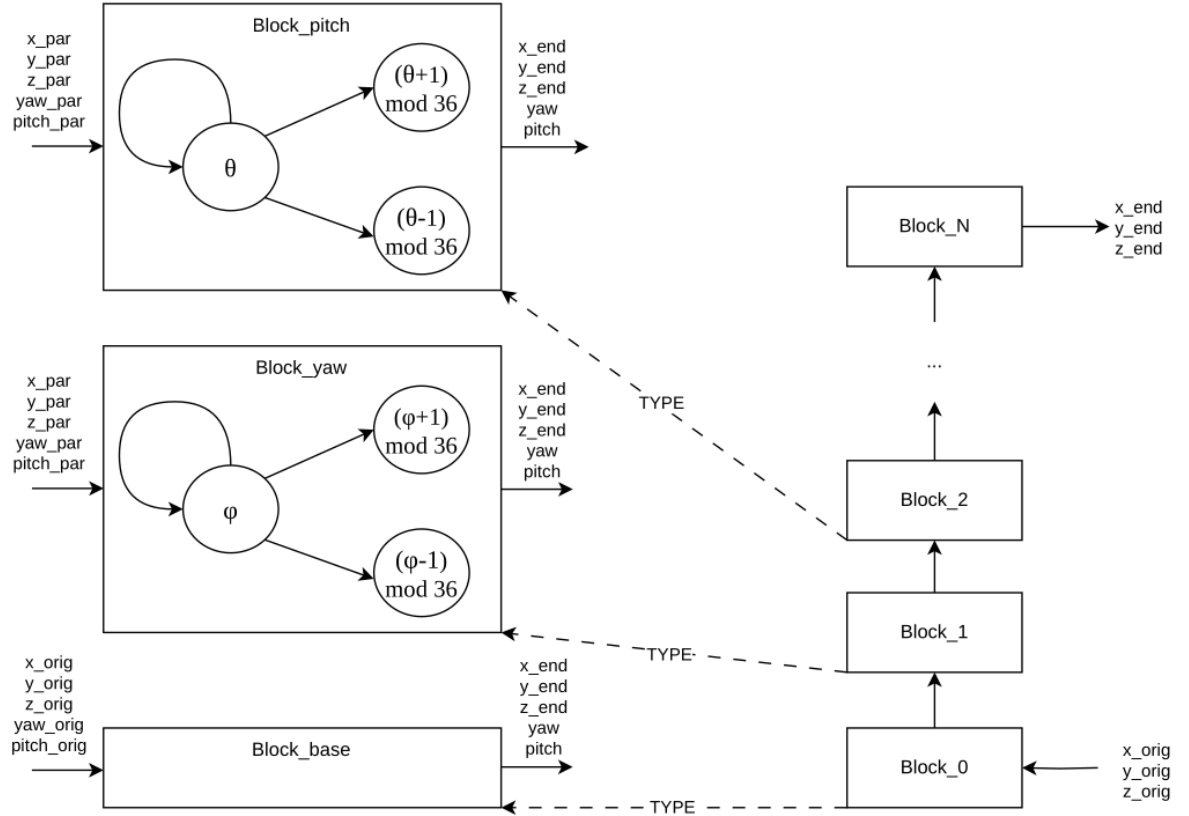
Figure 5.2: Robot configuration NuSMV model
