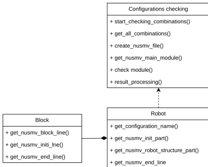
Figure 5.9: Class diagram of searching for relevant configurations
