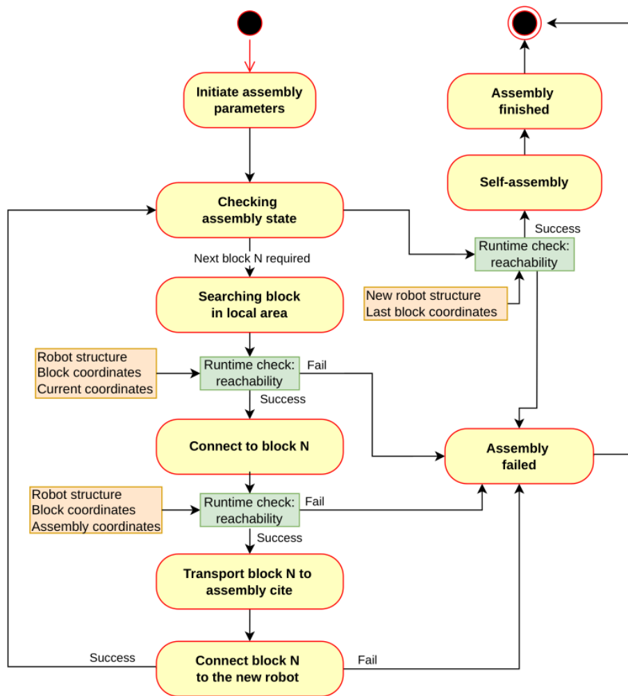
Figure 5.4: Self-replication process with potential model checking stages
