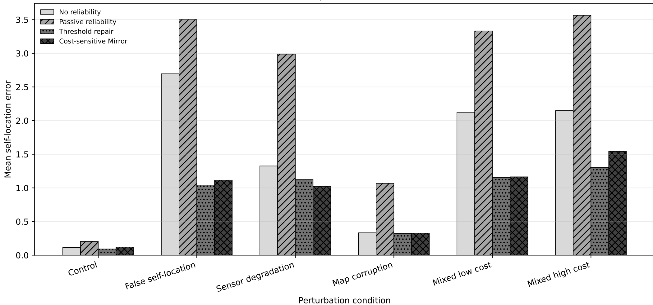
Self-model error by condition and architecture
