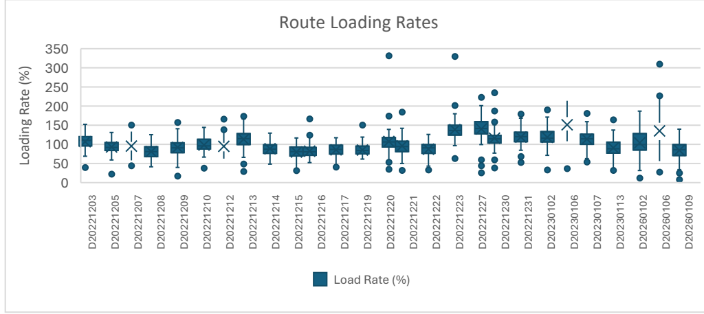
Figure 2. Distribution of route loading rates for original route instances.
