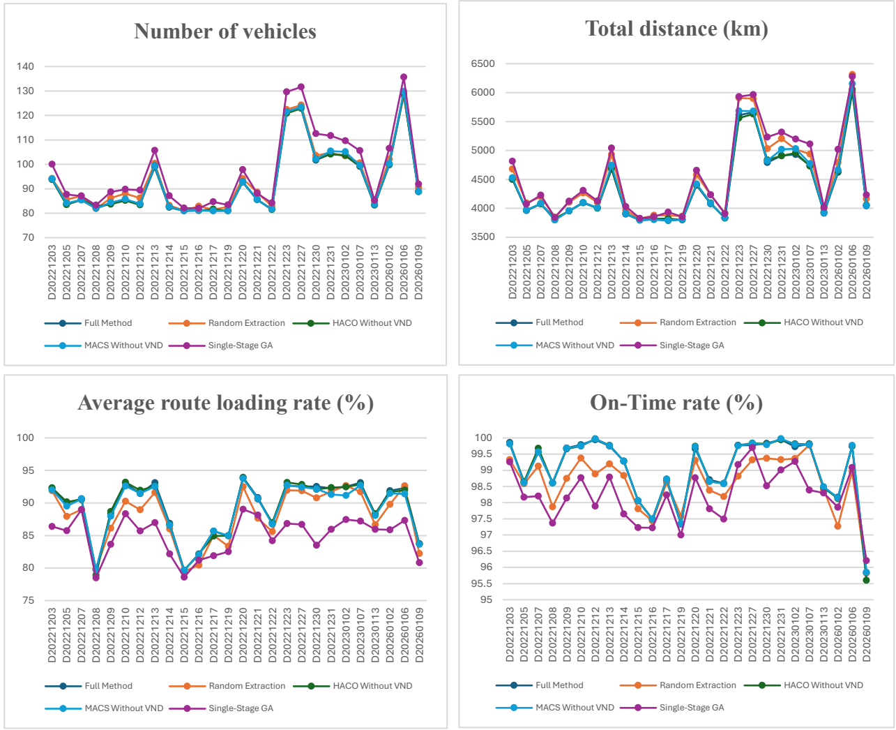
Figure 7. Comparison of routing performance for different instances
