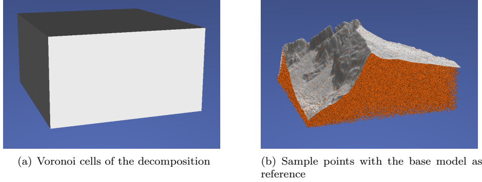
Figure 4.3: Result of the voronoi decomposition without cutting the boundary cells vs. the samples used for the decomposition with the base model as reference
