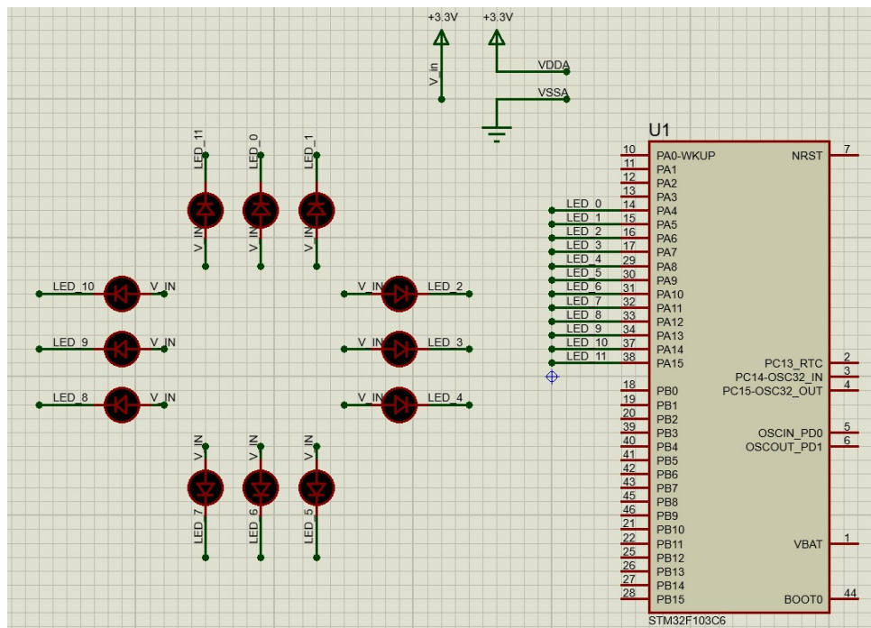
Figure 2.10: Proteus schematic for clock by using 12 red LEDs
