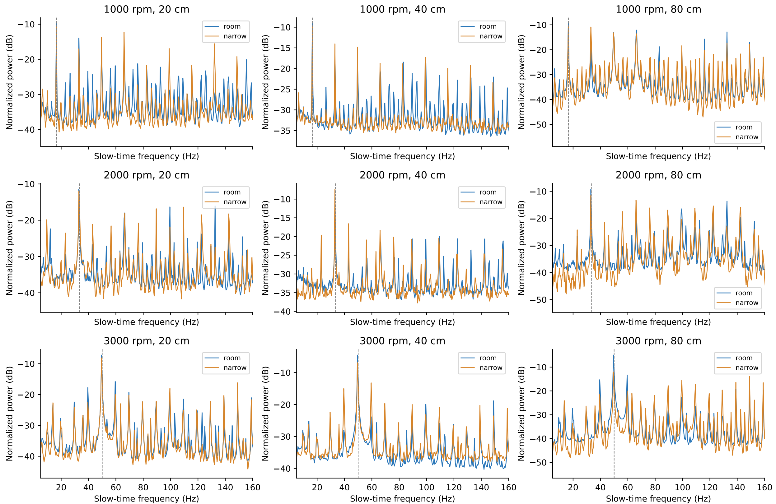
Masked harmonic-LS IQ spectra; frame coherence is an assumption; dashed: nominal shaft rate
