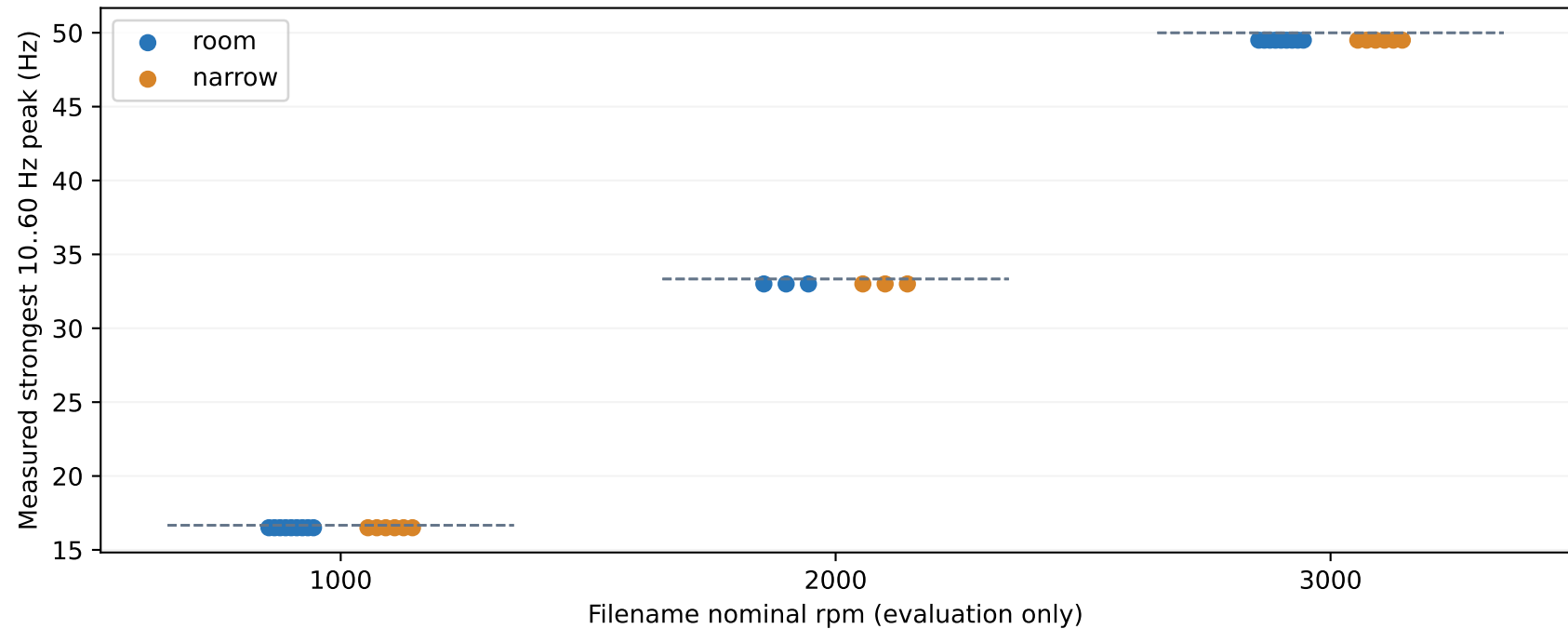
Physical sanity check; dashed lines are nominal shaft rates
