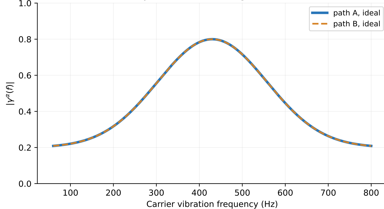
C. Ideal cyclic coherence magnitudes coincide
