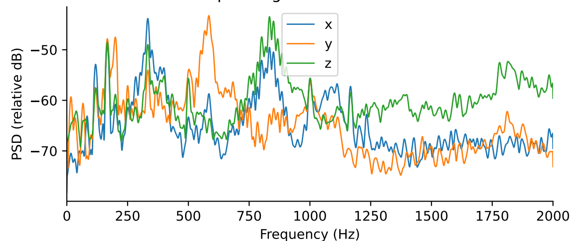
2000 rpm: segment-wise Welch PSD
