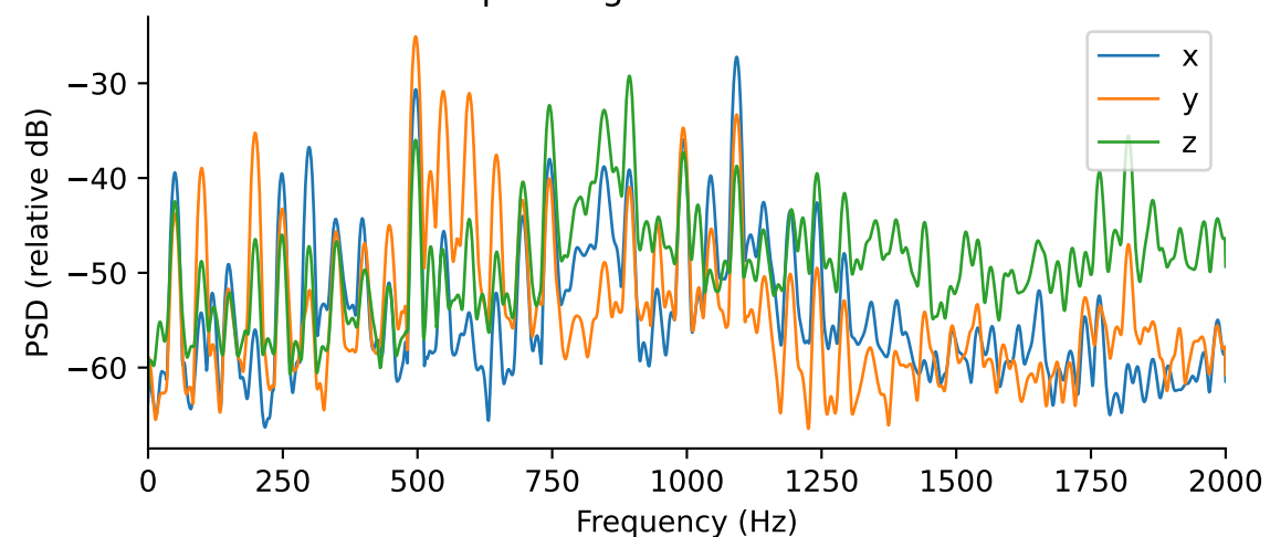
3000 rpm: segment-wise Welch PSD
