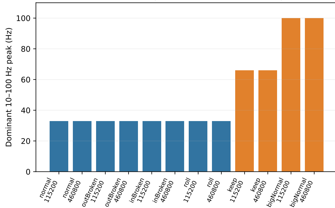
contact dominant peak, not confirmed shaft speed
