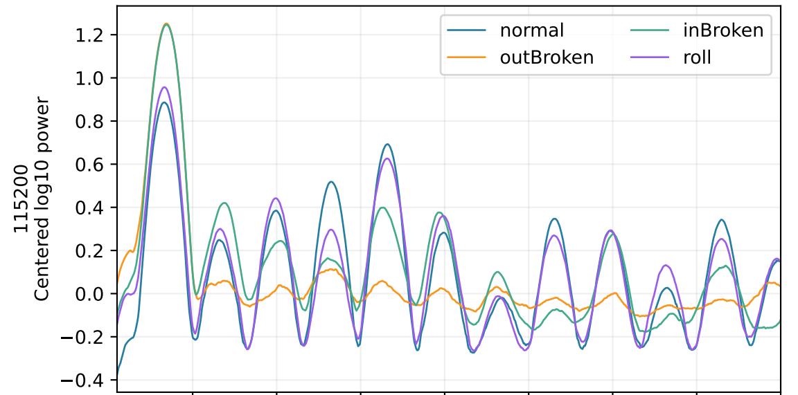
Within-frame IQ spectrum (resolution \approx 10.4 Hz)
