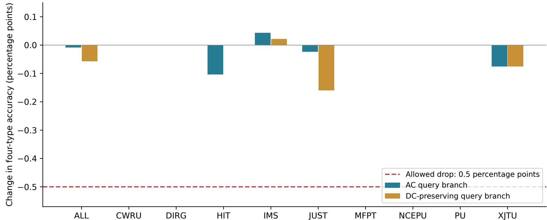
Conservative shared head: original-data regression by source dataset
