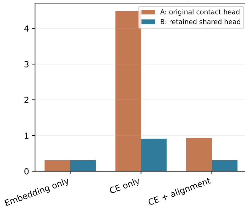
Standardized embedding MSE
