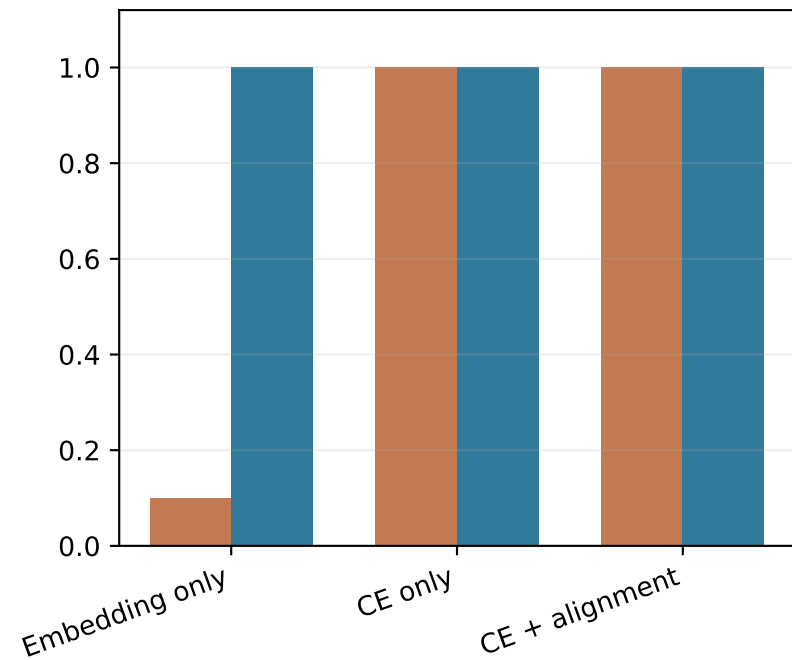
File macro-F1
